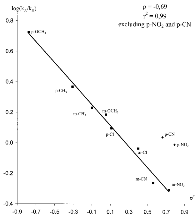
Figure 4. Substituent effects in the aerobic oxidation of substituted benzyl alcohols under NHPI catalysis
