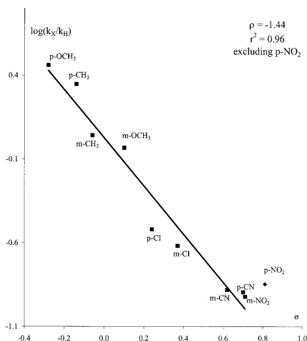
Figure 1. Substituent effects in the aerobic oxidation of substituted benzyl alcohols under TEMPO catalysis
