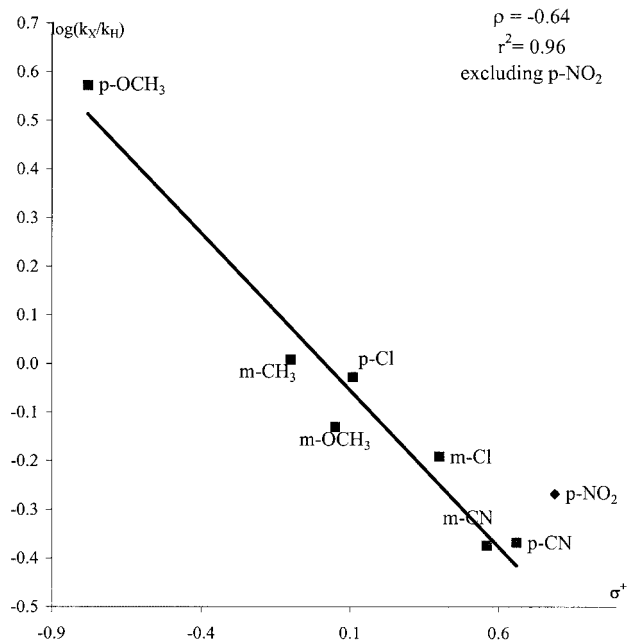
Figure 3. Substituent effects in the aerobic oxidation of substituted benzyl alcohols using 3 as a catalyst in the presence of p -toluenesulfonic acid
