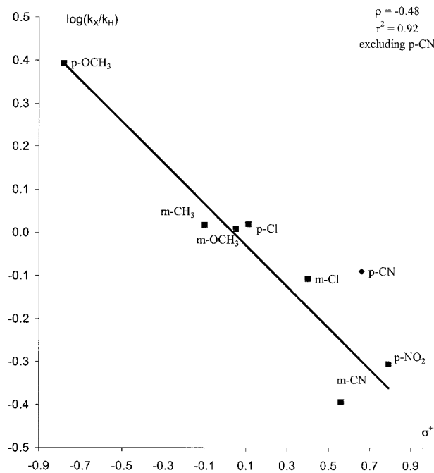
Figure 2. Substituent effects in the aerobic oxidation of substituted benzyl alcohols using 3 as catalyst
